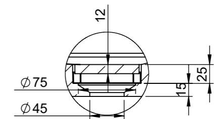
DETAIL AQ SCALE 1 : 5
